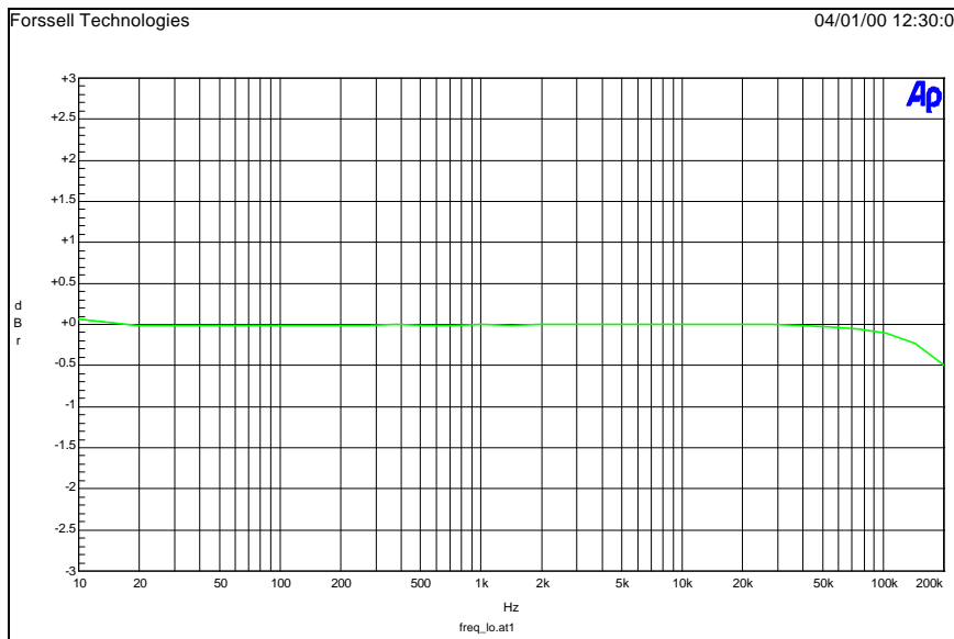
Wide band Freq Response
