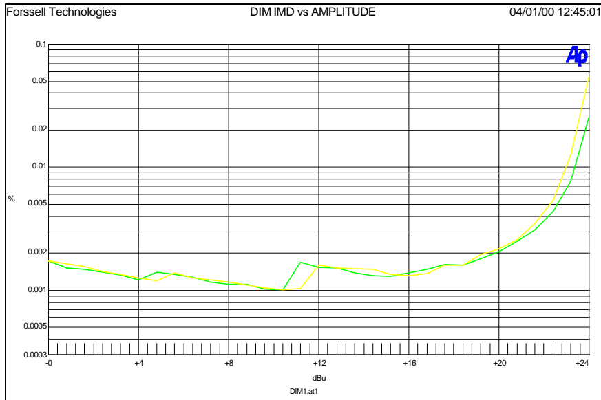
DIM (dynamic) Distortion vs Output Amplitude. Green = 10k, Yellow = 600 ohm Load
