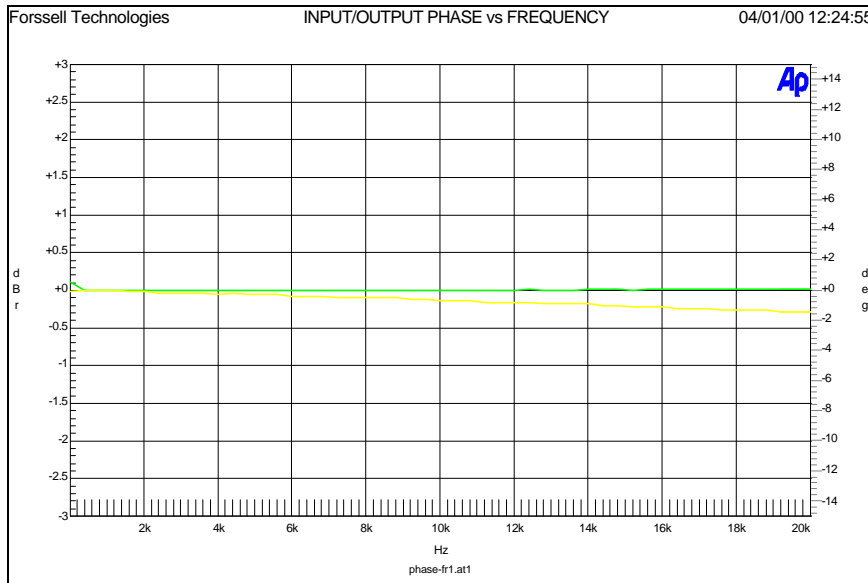
Phase/Freq Response
