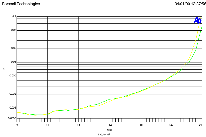
THD+N vs Output Amplitude 10k Load = green, 600 ohm Load = yellow
