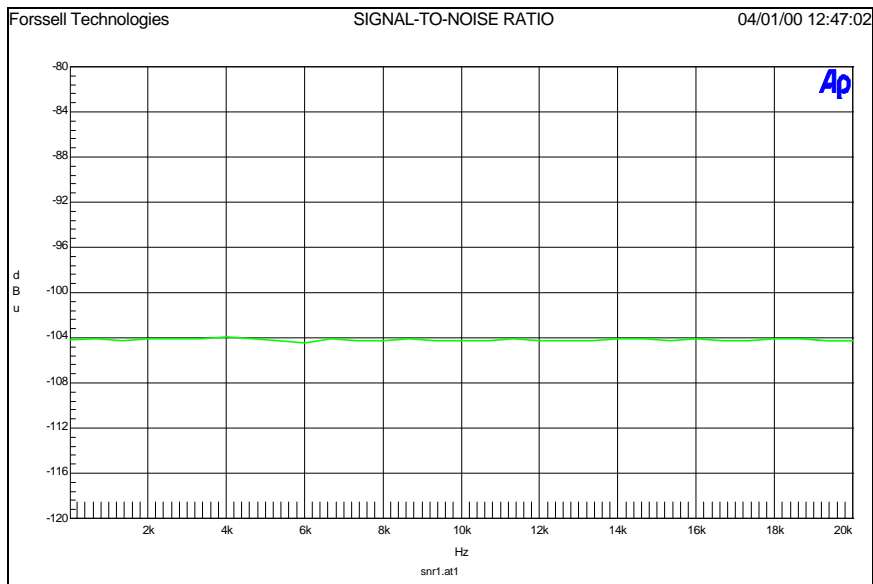
22 - 22 KHz Bandwidth Noise Floor
