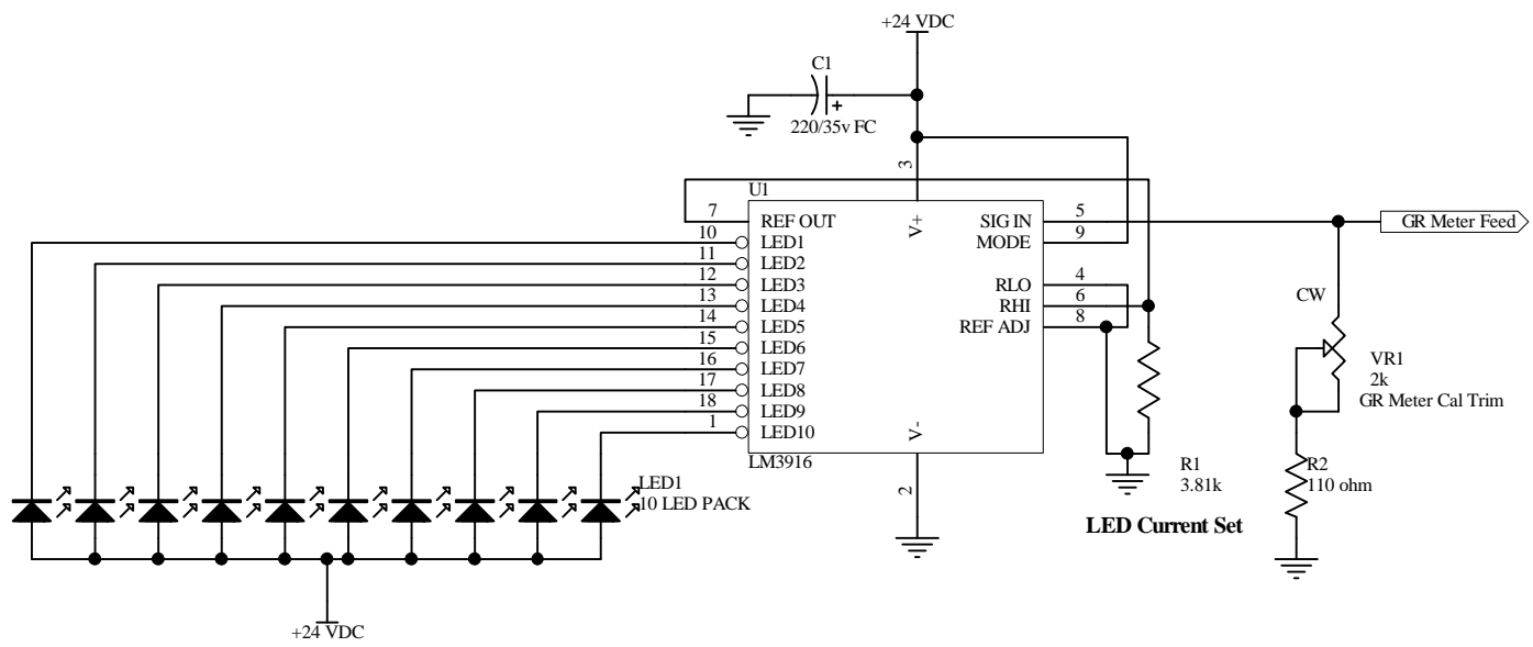
Opto Compressor LED Array Metering Circuit
