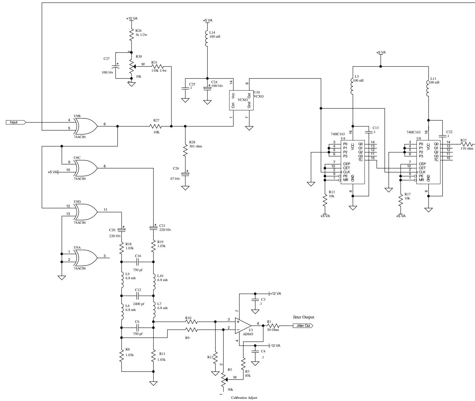
Jitter Detector Output Section
