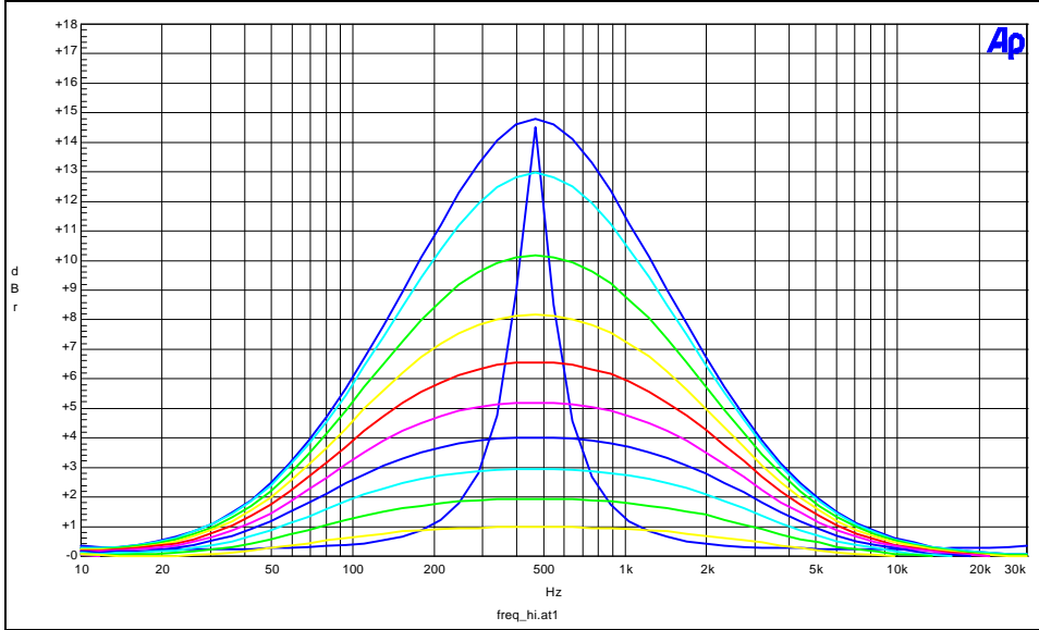
EQ Freq Resp for each Boost Control Step Position (Hi Q shown Max Boost only)
