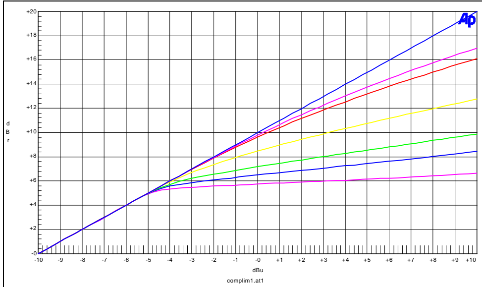
Compressor Slope w/Ratio set at 5, 3, 1, 11, 9, 7 o'clock positions & off
