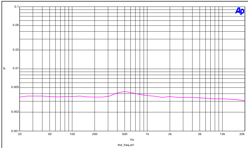
THD+N (%) vs Freq with 600 Ohm Load at 0 dBu Output
