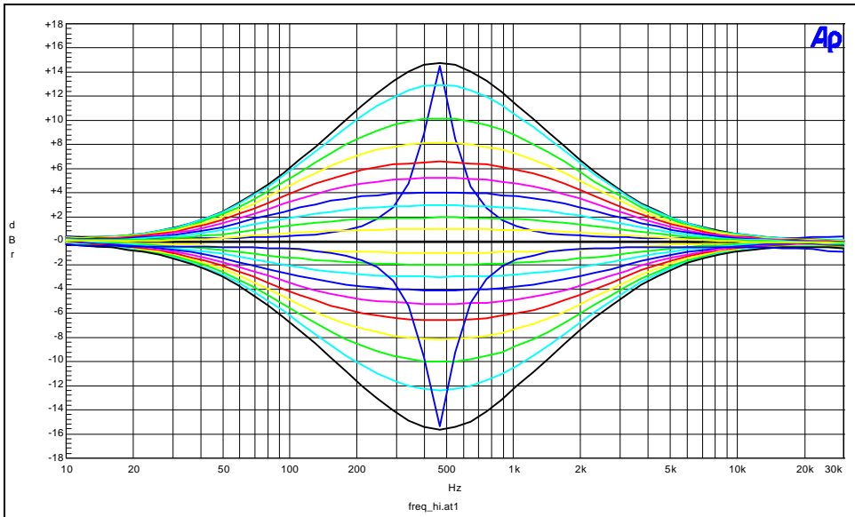
EQ Boost/Cut Response for each Step Position of Boost/Cut Control
