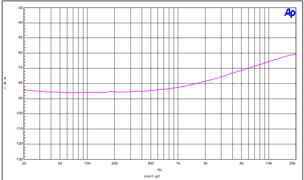
Common Mode Rejection at 30 dB gain. CMRR ratio @ 1 KHz= 112 dB
