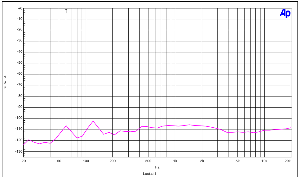
1/3 Oct Noise Floor with CS-1 Set to Unity Gain Line In to Line Out (note... This test data was taken with the PCB not mounted in an enclosure. )
